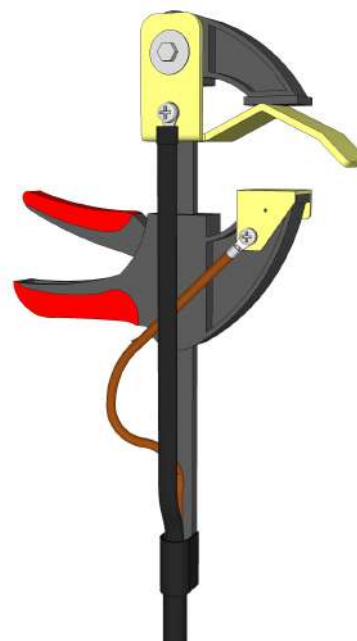
Overhead line Kelvin connection clamp
